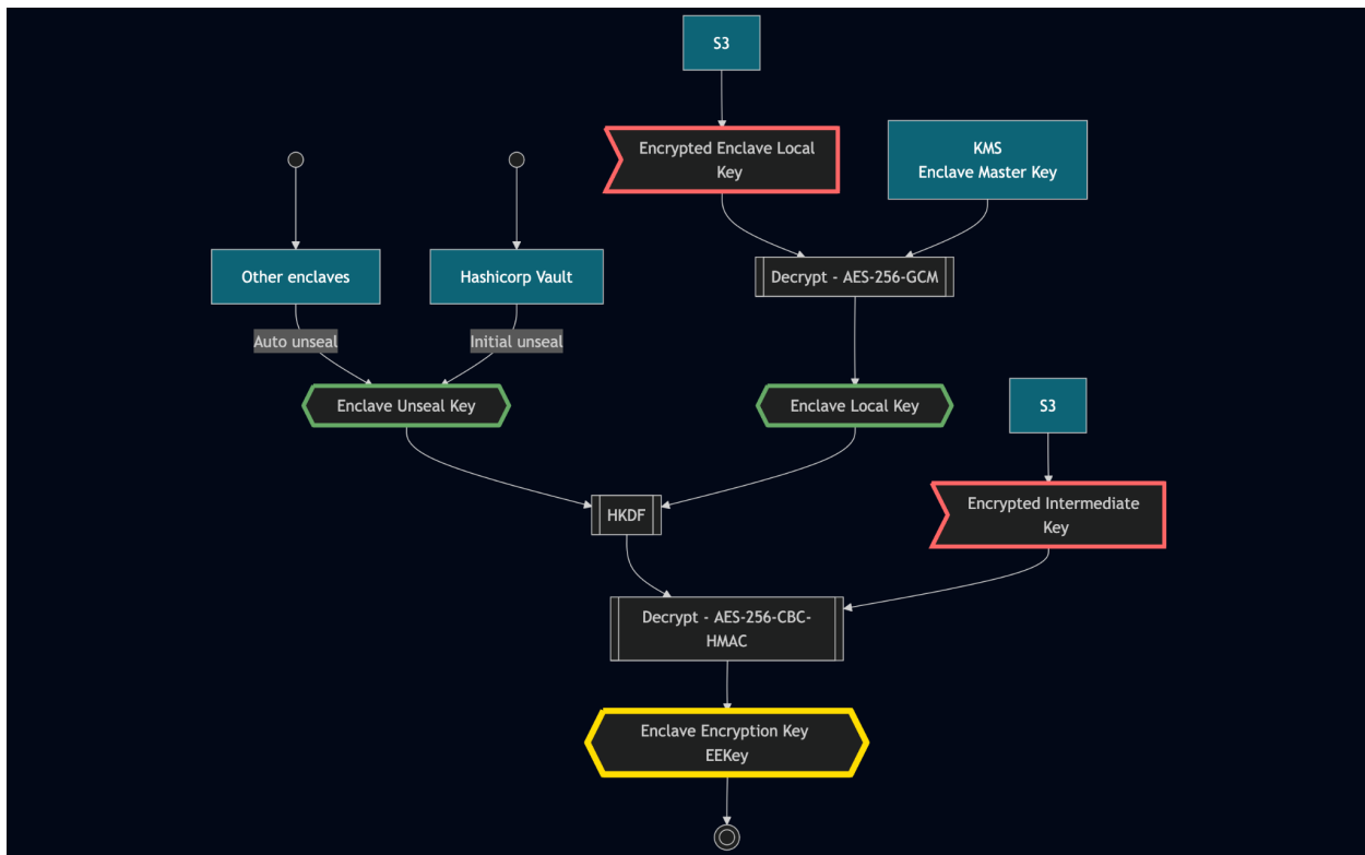
Figure: How keys are used to decrypt the Enclave Encryption Key
