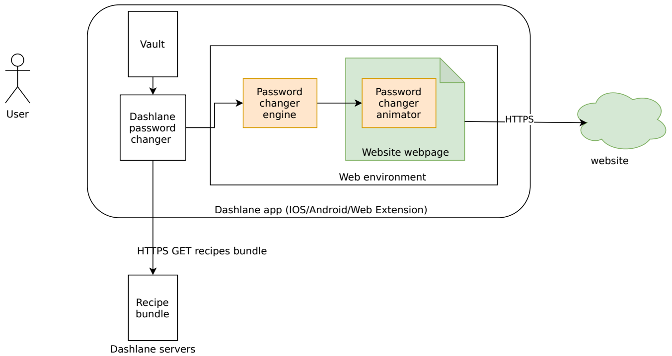
Figure 6: Password Changer Structure
